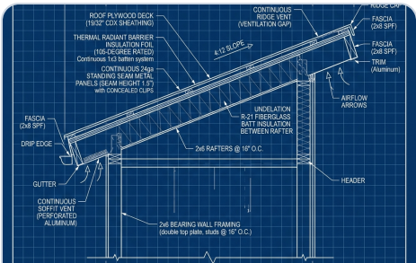
3. 105°F RADIANT ROOF
