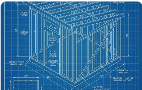
2. 2X4 KILN-DRIED FRAMING
